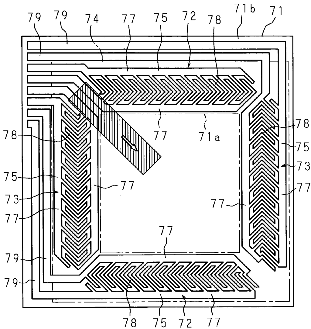
FIG. 2 PRIOR ART
